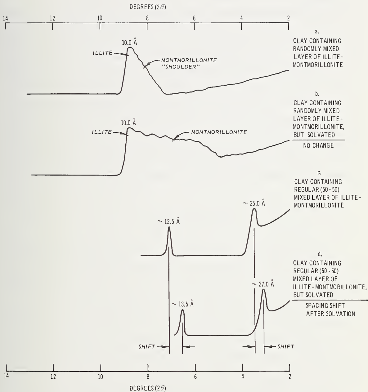
Figure 36. X-ray diffractograms of clays containing mixed-layer illite-montmorillonite.
